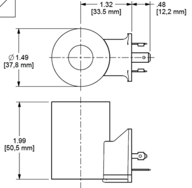
AC COIL
