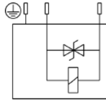
DC COIL (with TVS Diode)
