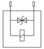
DC COIL (With TVS Diode)
