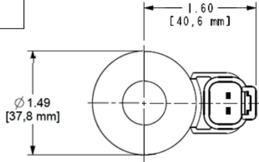
DC COIL
