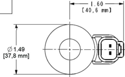
DC COIL
