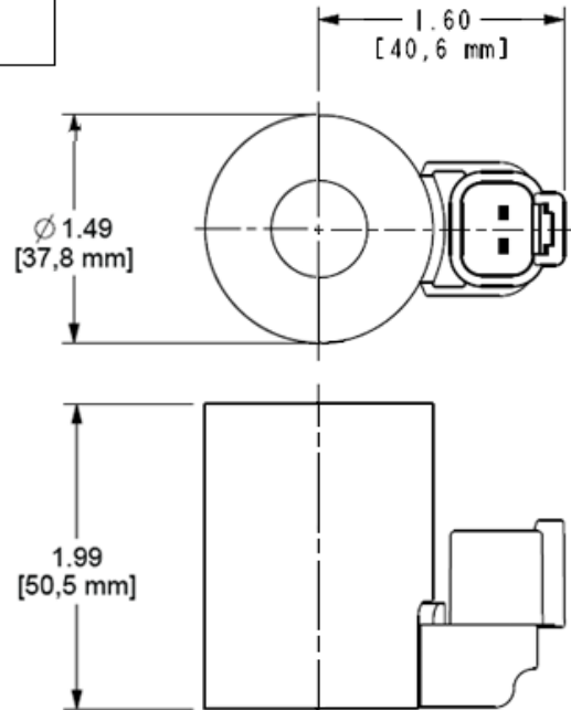
DC COIL
