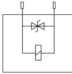
DC COIL
