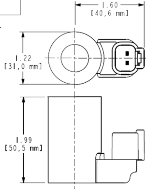
DC COIL
