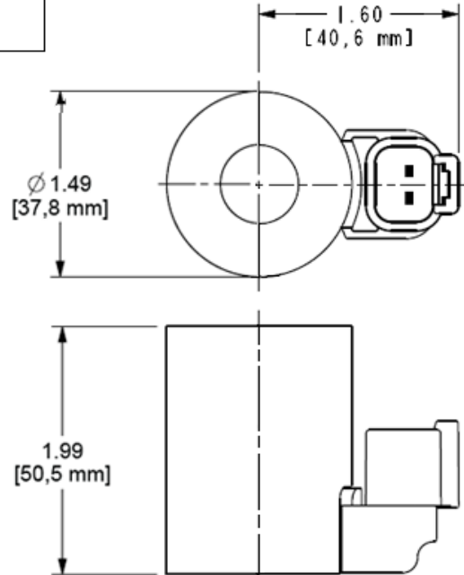
DC COIL
