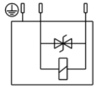
DC COIL (with TVS Diode)
