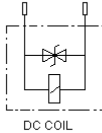
DC COIL
