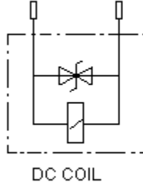
DC COIL
