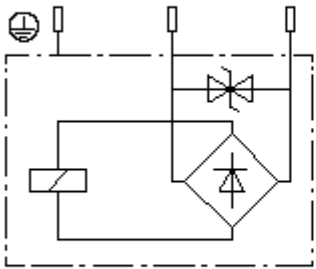
AC COIL
