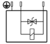
DC COIL (with TVS Diode)
