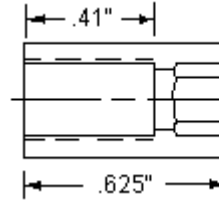
Internal Hex Size 5/32" U.S.
