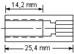
Internal Hex Size 5 mm metric
