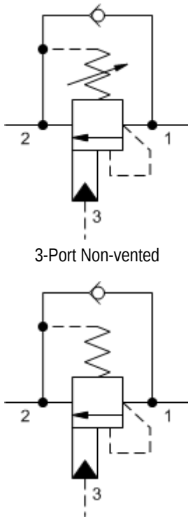
3-Port Non-vented, Fixed Setting
