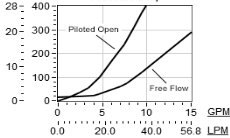
BAR PSI Free Flow and Piloted Open Pressure Drop
