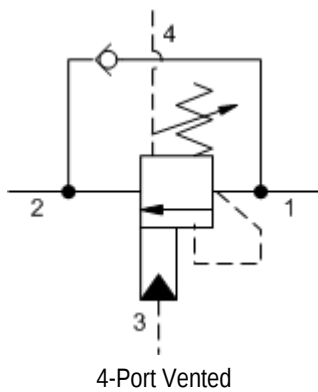
4-Port Vented
