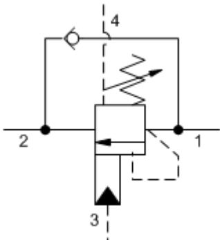
4-Port Vented
