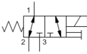
M-Control, H-Spool
