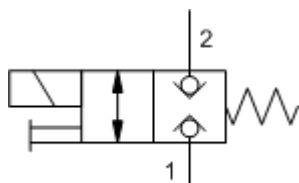
M-Control, C-Poppet
