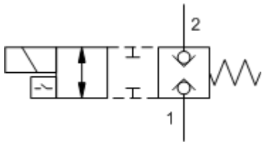
Z-Control, C-Poppet
