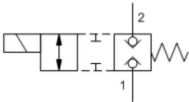
X-Control, C-Poppet
