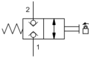
L-Control, C-Poppet
