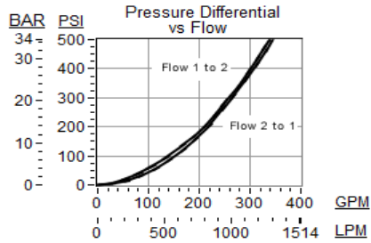
Model LOKB8 installed in T-19A Cavity
