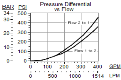
Model LOKB8 installed in T-19AU Cavity
