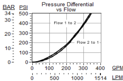
Model LOKB8 installed in T-19A Cavity
