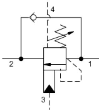
4-Port Vented
