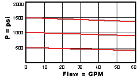
Regulated Pressure
