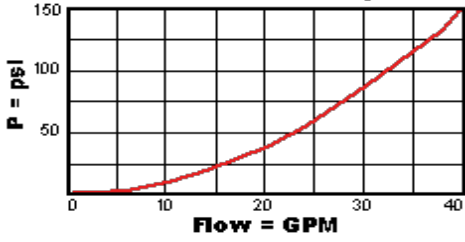
No Load Pressure Drop with Valve Full Open
