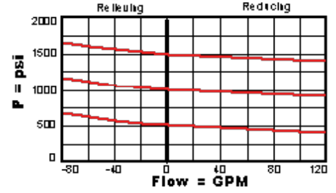
Regulated Pressure
