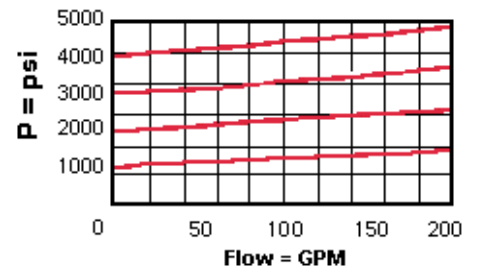
Typical Pressure Rise
