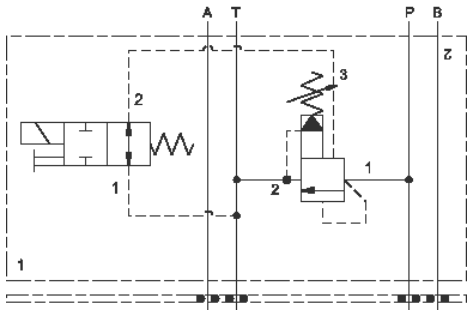
Normally Open
